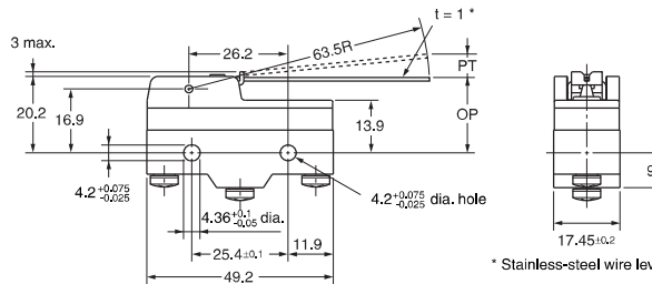
* Stainless-steel wire lever
